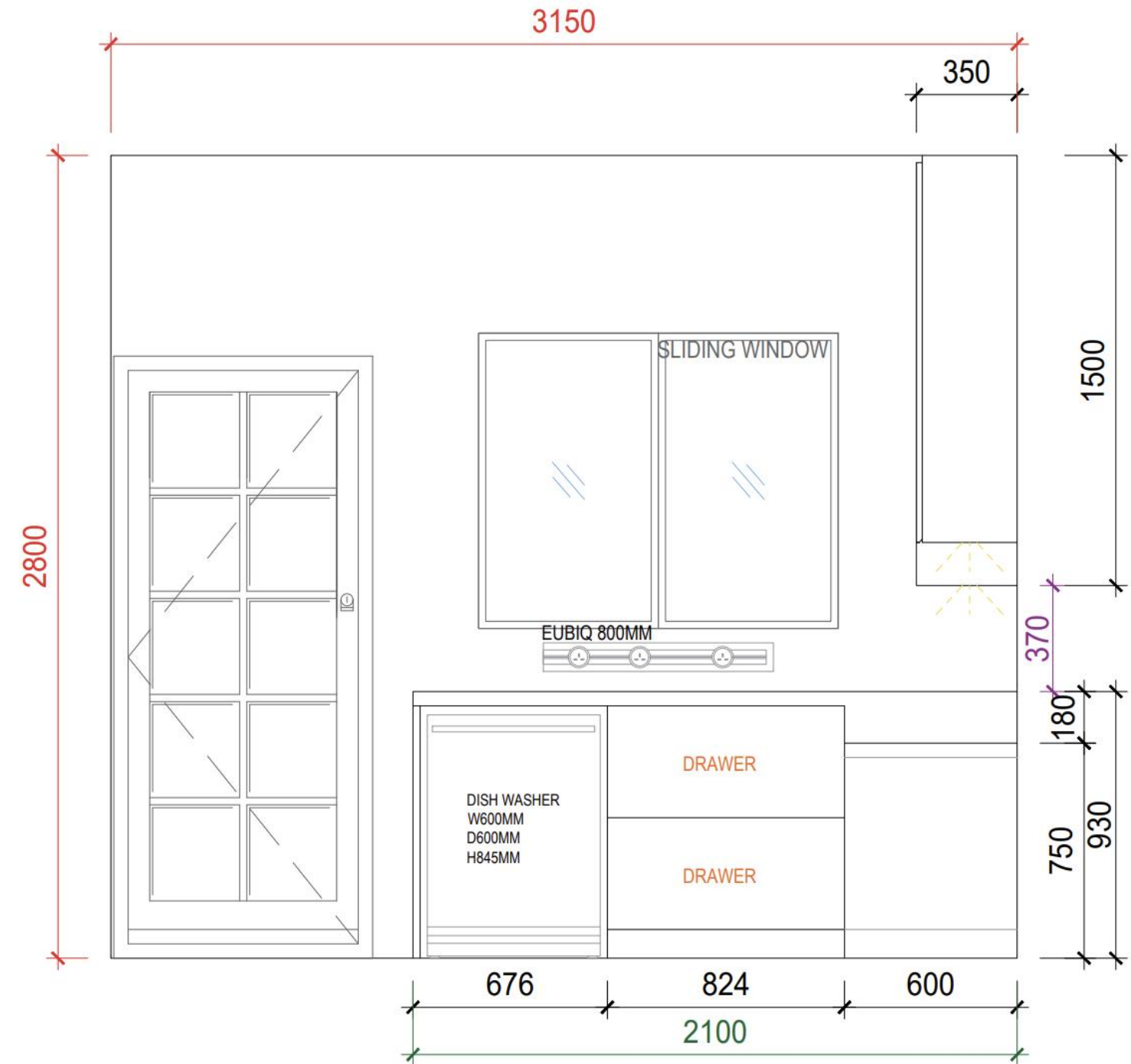
WET KITCHEN ELEVATION -A 1:10
