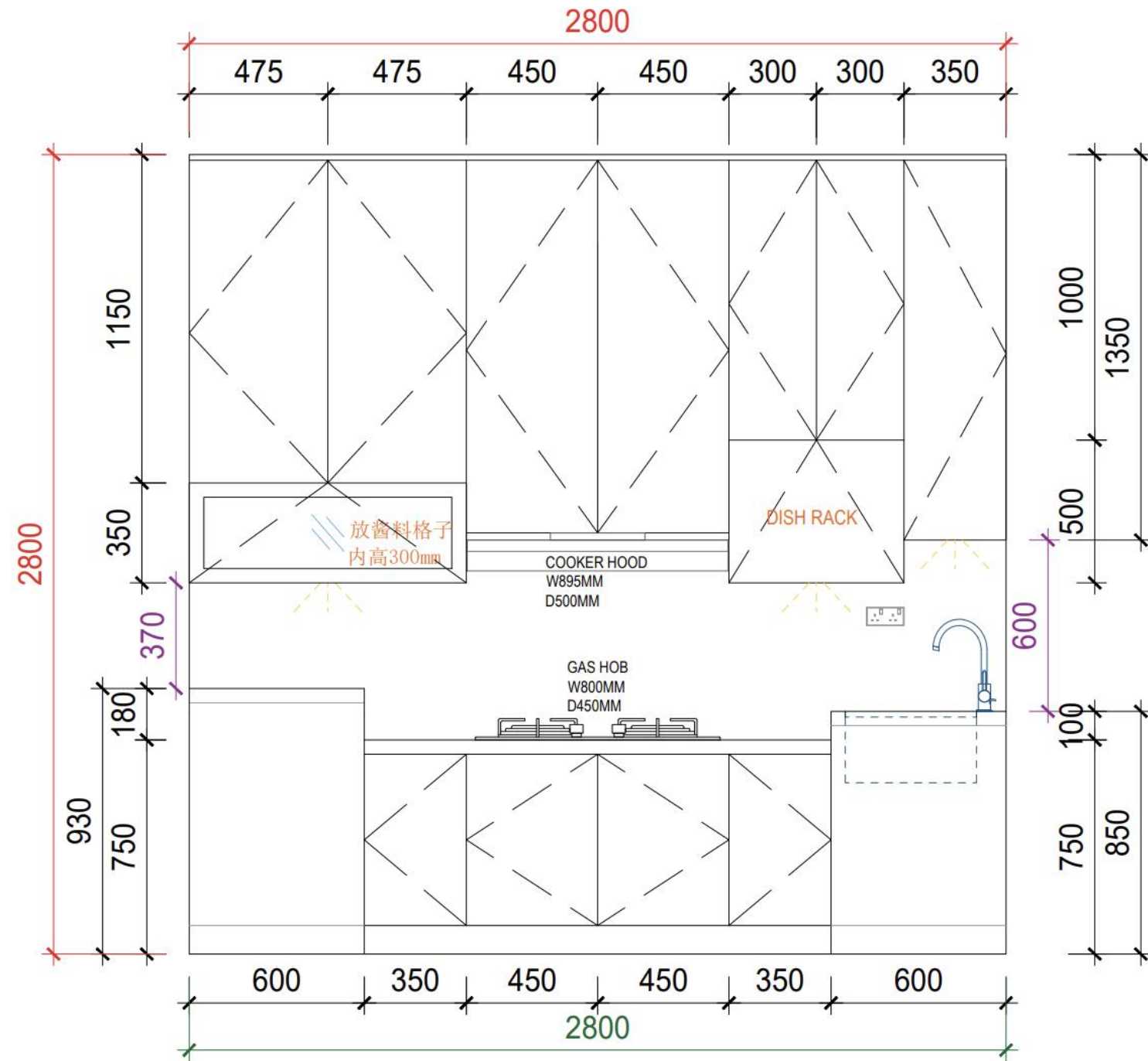
WET KITCHEN ELEVATION -B 1:10
